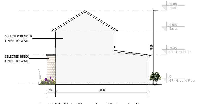
② H03 Side Elevation (Extended) 1 : 200
