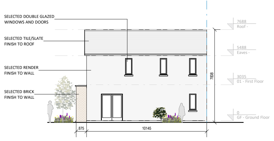
④ H03 With Bay Window Rear Elevation 1 : 200
